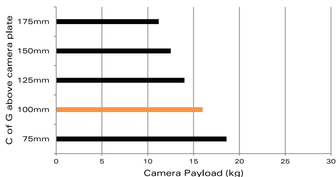
Payload Range
