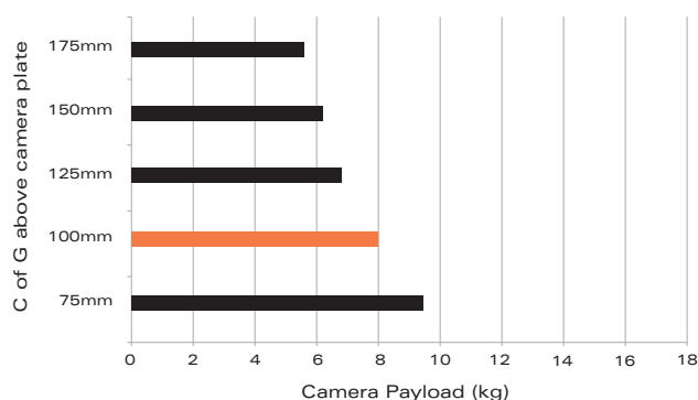
Payload Range
