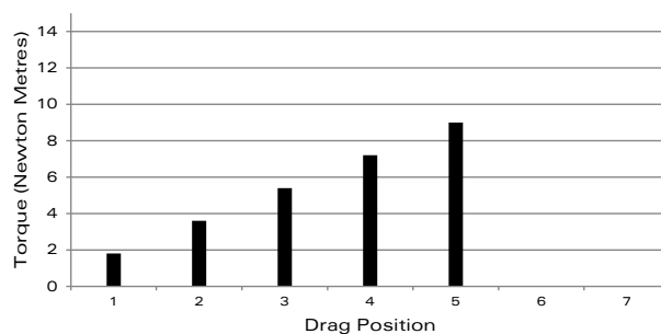
Drag Torque
