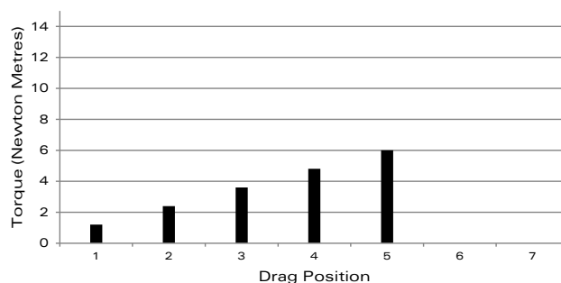
Drag Torque
