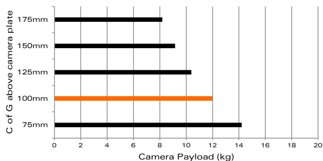
Payload Range
