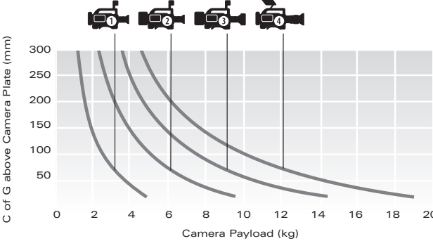
Counterbalance Performance
