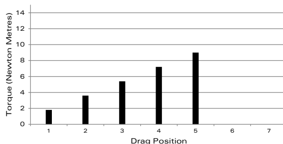
Drag Torque
