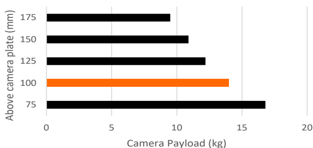
Payload Range (ArtX 7)
