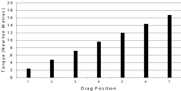
Drag Torque
