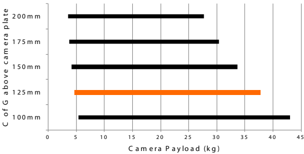
Payload Range
