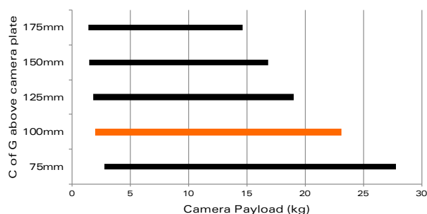
Payload Range
